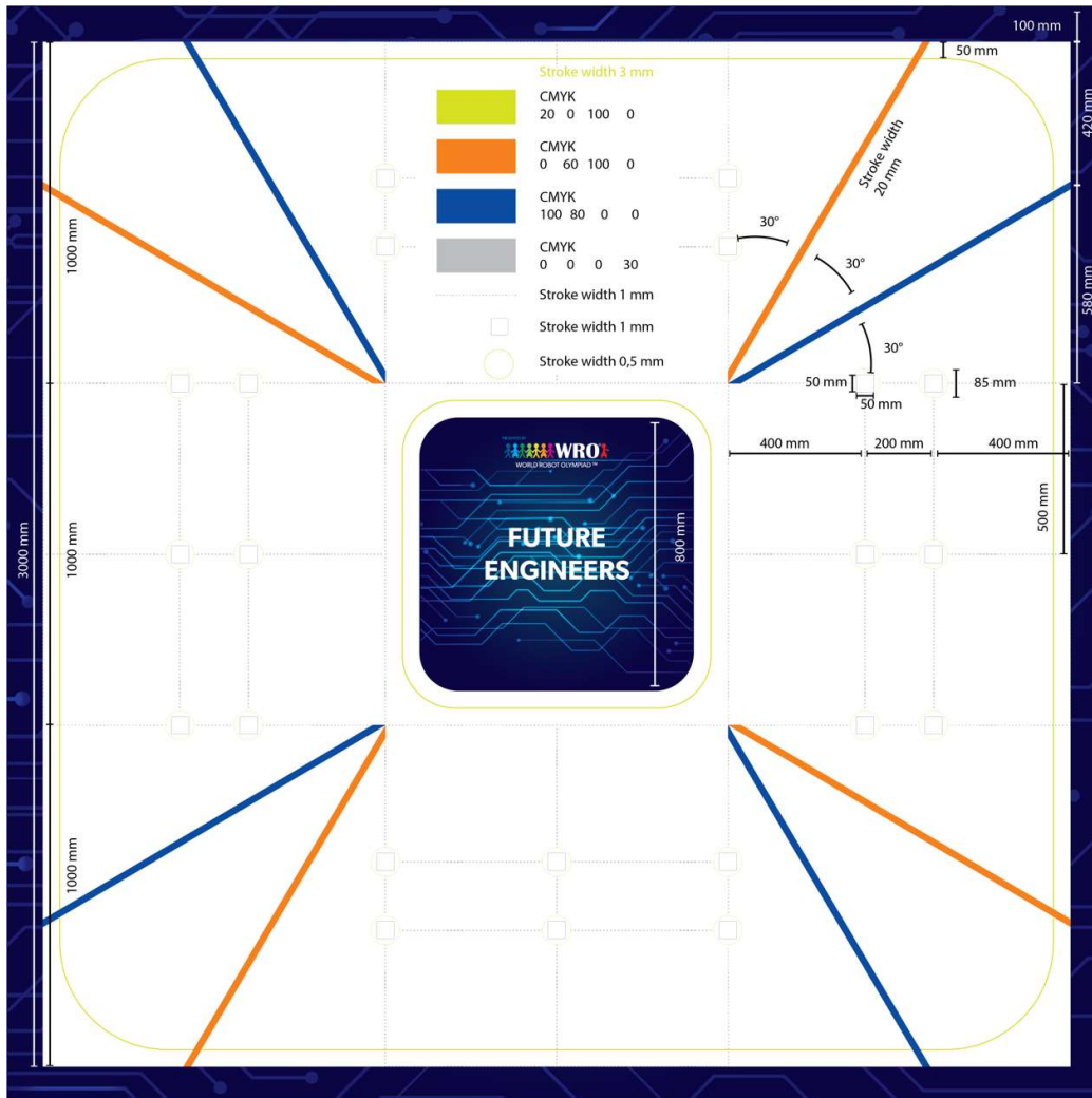
Figure 11: The game field map with sizes
